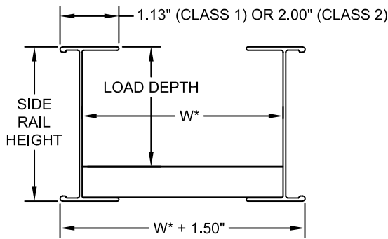
TRAY CROSS-SECTION
