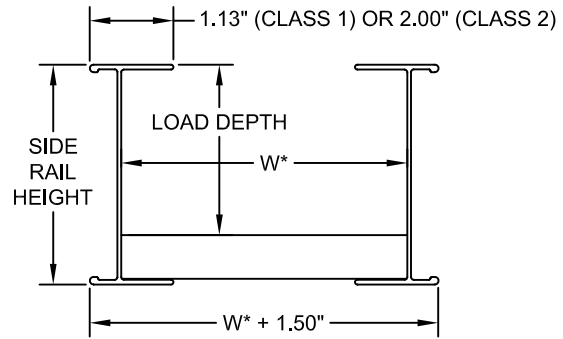
TRAY CROSS-SECTION
